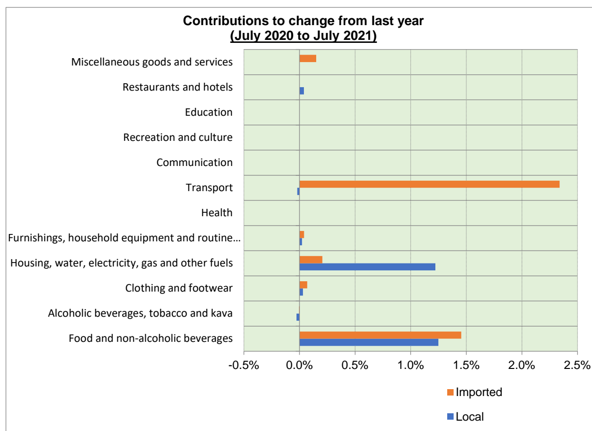
Figure 4 Contributions to % change from last year, all groups: July 2020 to July 2021
